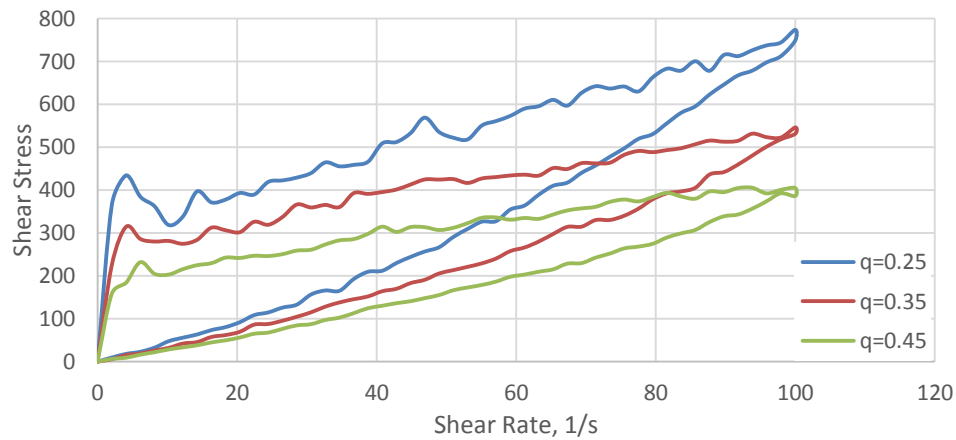
Figure 25. Flow curve for three mixes with q = 0.25, 0.35 , and 0.45
